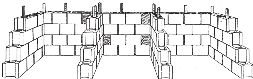
FIGURE 2. 3-bin concrete block composter
