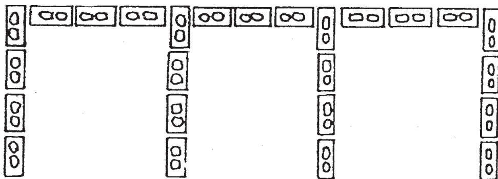
FIGURE 4. First layer of concrete blocks for the 3-bin unit
