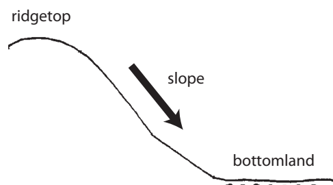
Figure 4. Ridgetops and slopes tend to shed water, while soils at the bottom of slopes and in low areas collect water.
