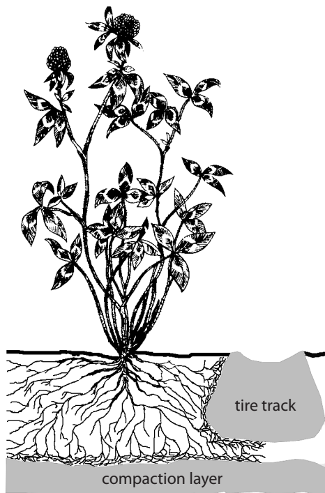
Figure 3. Compacted soil resists root penetration and water movement.
