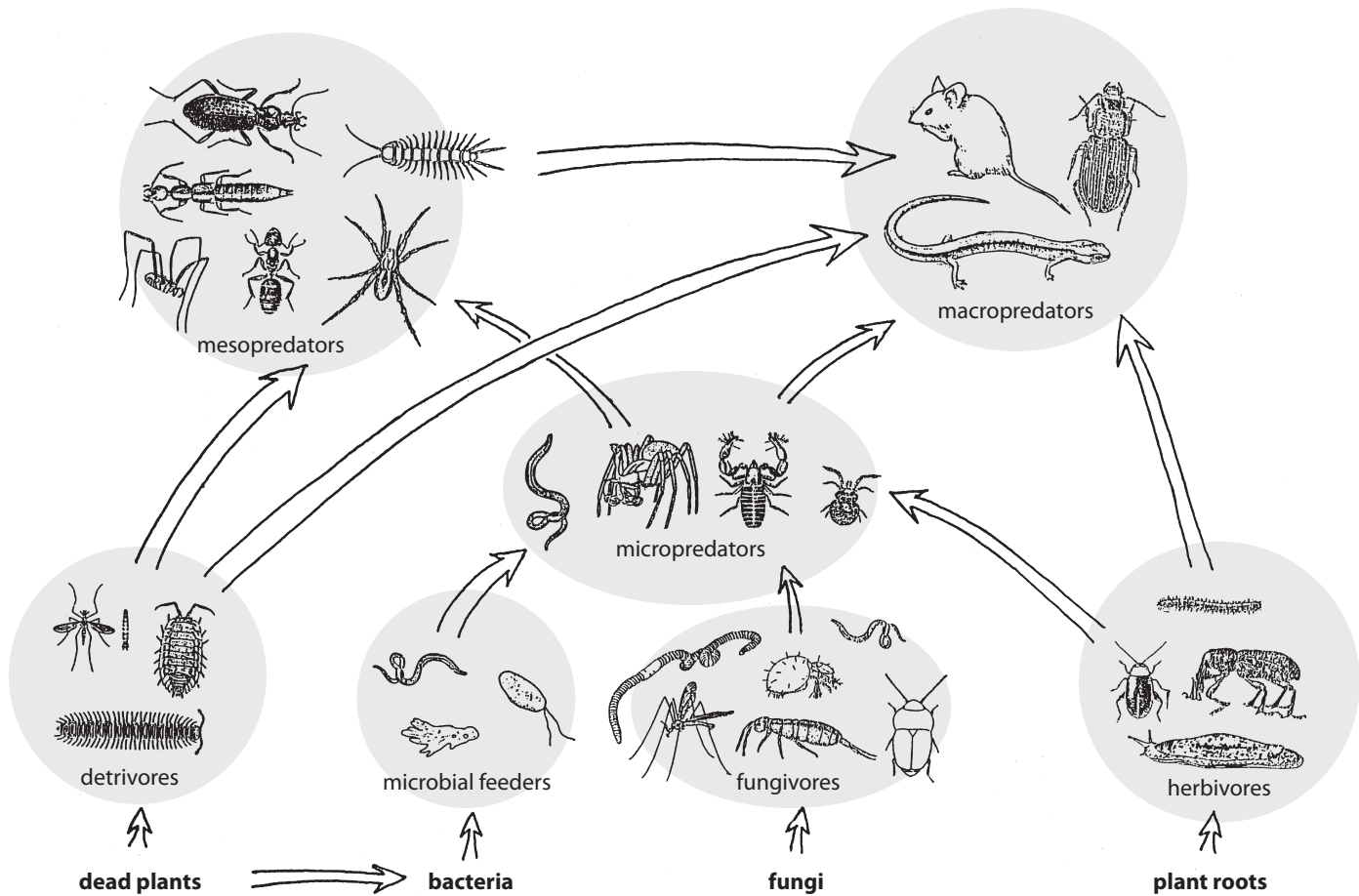
Figure 5. The soil food web.
