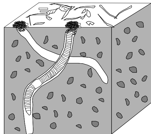
Figure 6. Earthworm channels create macropores, which improve a soil’s permeability and aeration.
