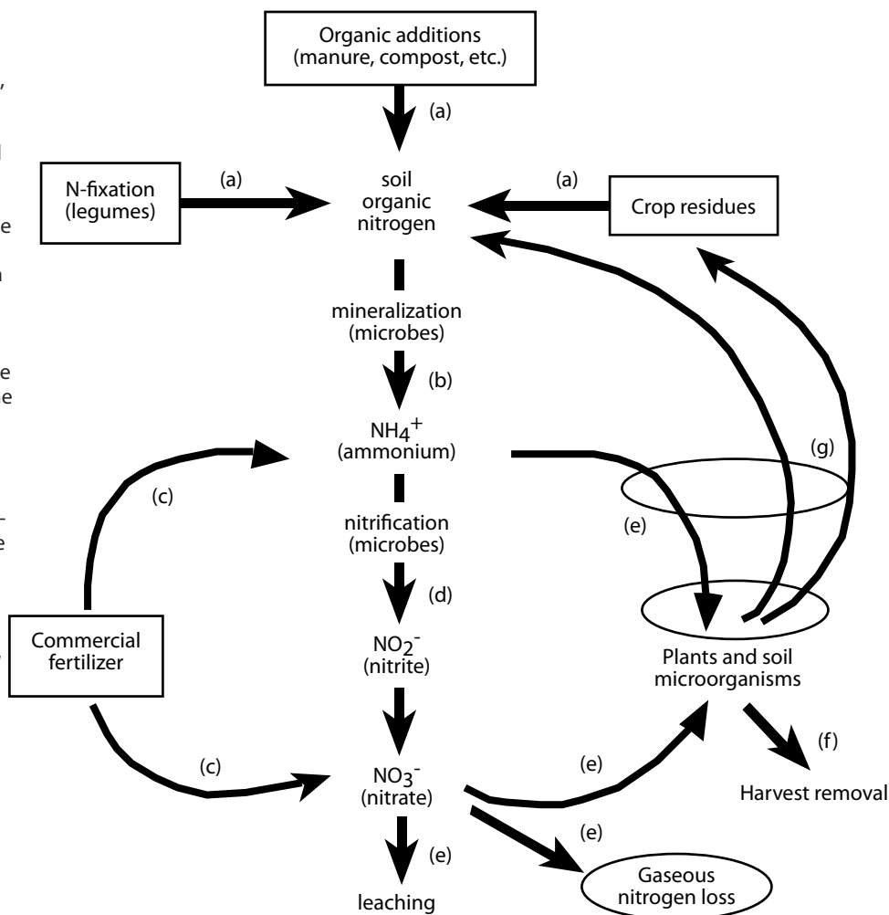
Figure 7. Nitrogen cycle:
