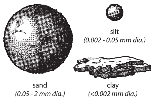
Figure 1. Shapes of soil particles.
