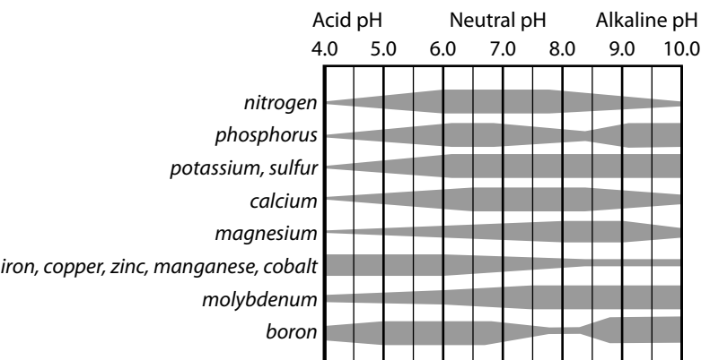
Figure 8. Effect of soil pH on the availability of plant nutrients.
